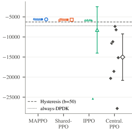
(b) All controllers, full scale; mean and 95% t-CI
