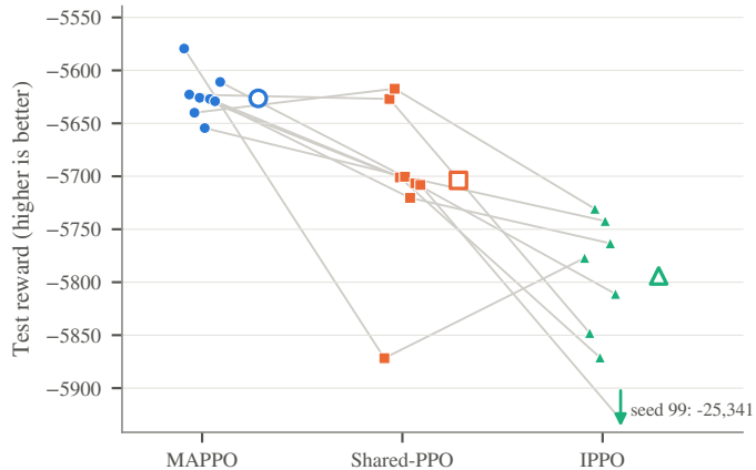
(a) Seed-matched runs (lines join equal seeds); open marker = median
