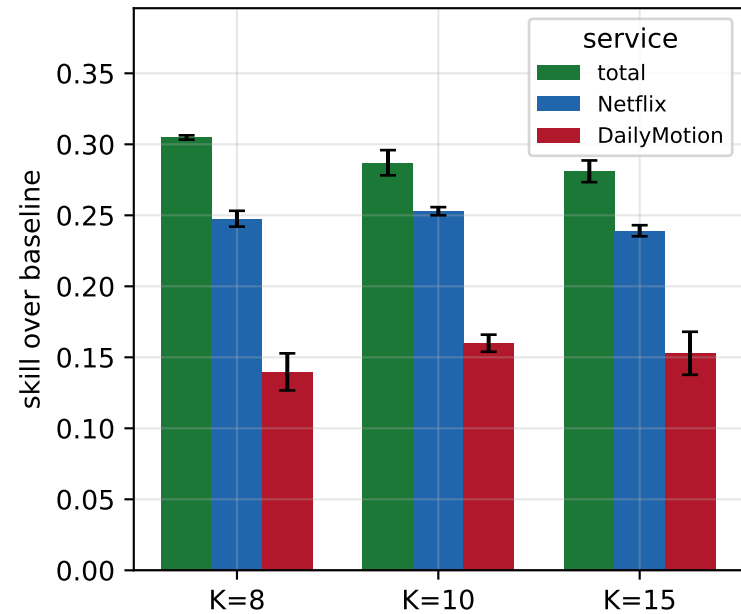
Generalization across traffic types vs. persistence vs. seasonal-naïve
