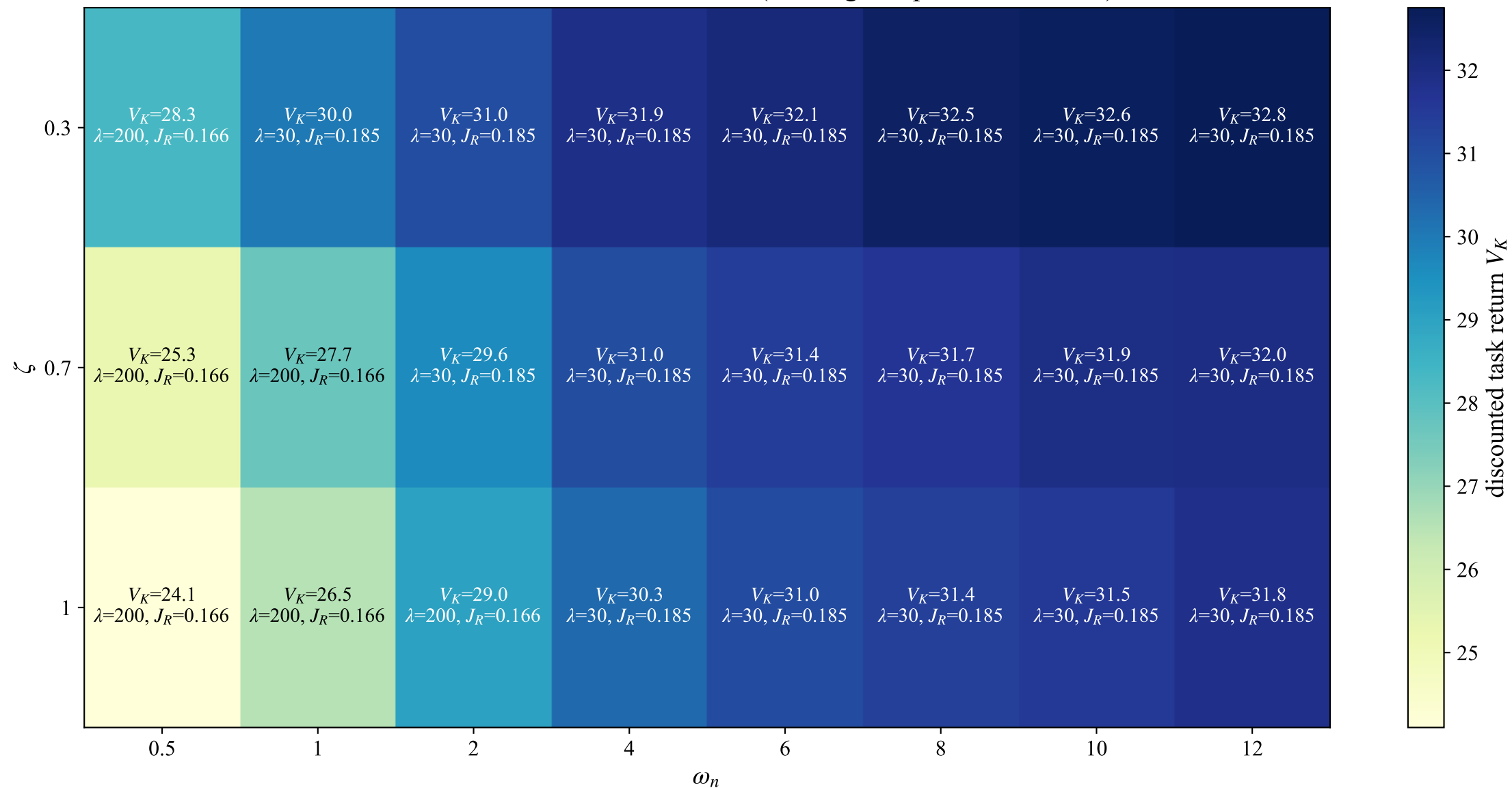
Best transfer discounted task return V_K (training samples = 1,572,864)
