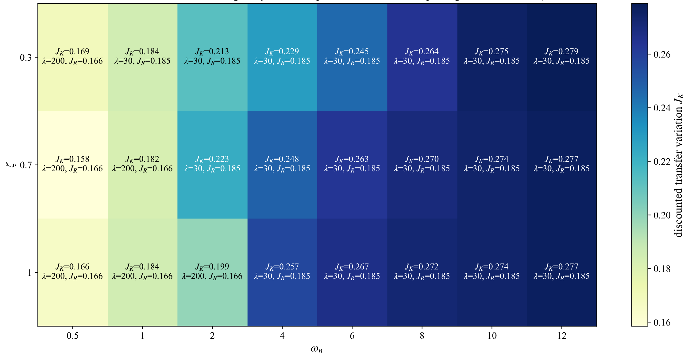
Transfer variation J_K of the policy achieving the best V_K (training samples = 1,572,864)
