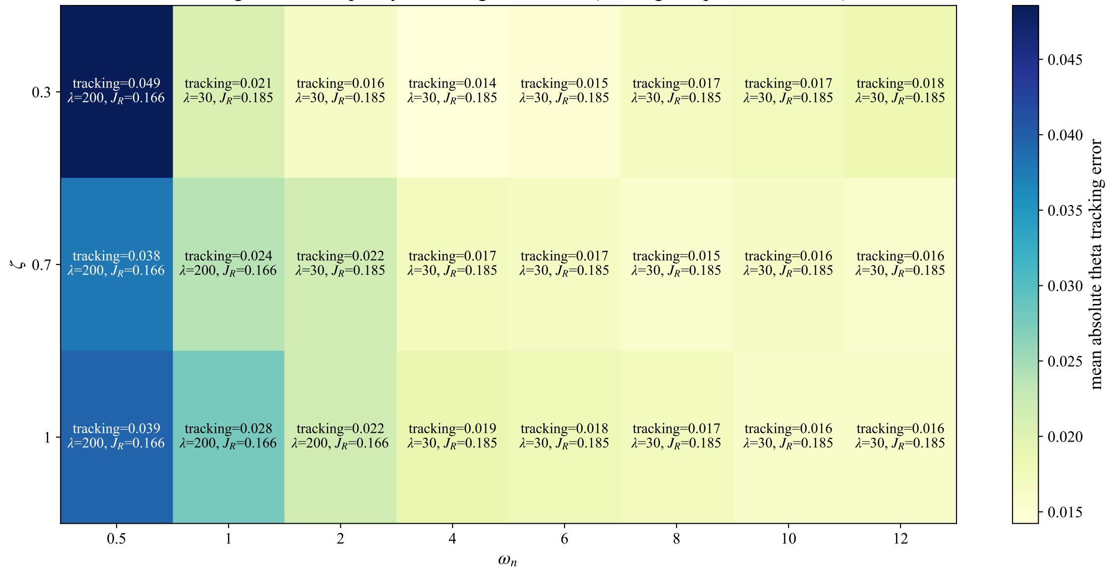
Tracking error of the policy achieving the best V_K (training samples = 1,572,864)
