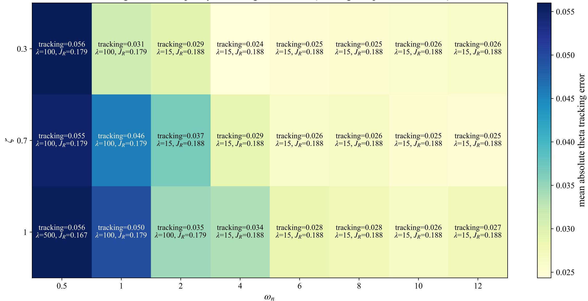
Tracking error of the policy achieving the best V_K (training samples = 1,179,648)
