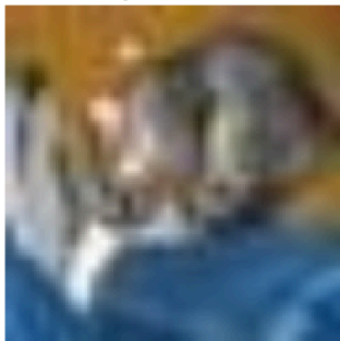
Original — score: 0.059
