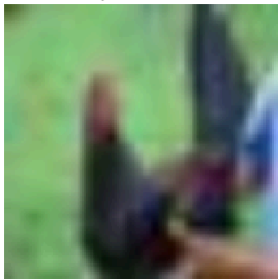
Original — score: 0.392
