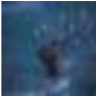
Original — score: 0.059
