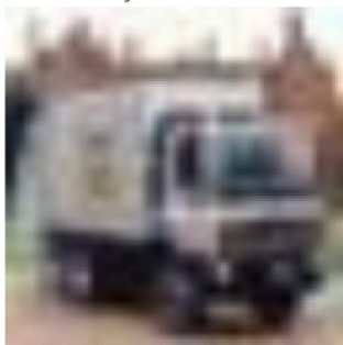
Original — score: 0.230
