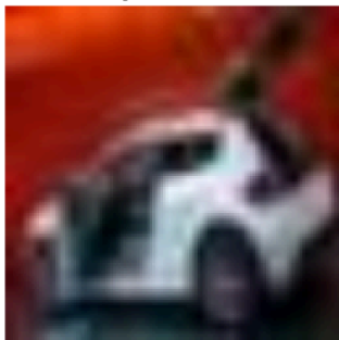
Original — score: 0.068
