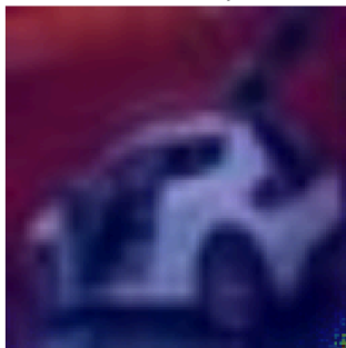
Grad-CAM Overlay
