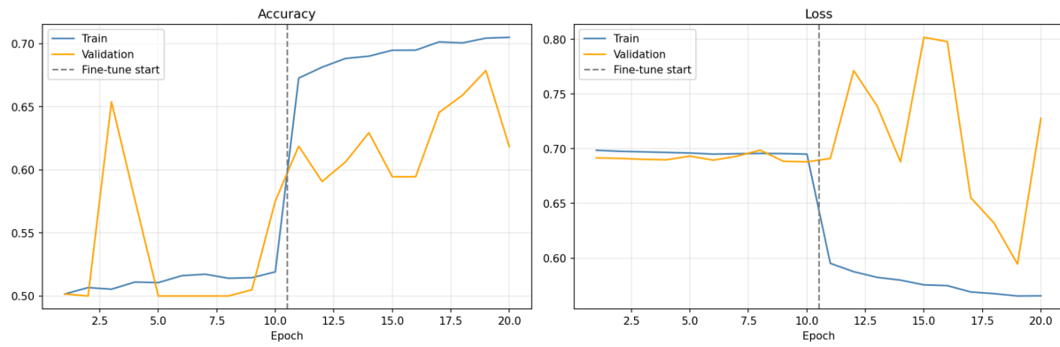
Baseline Spatial CNN — Training History
