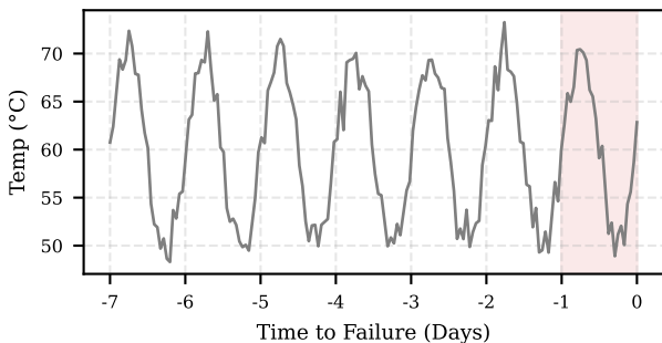
Macro Scale: 1 Week SCADA (Daily Cycles)
