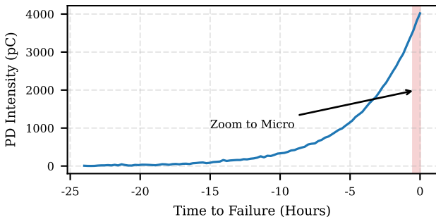
Meso Scale: Last 24 Hours PD (Exponential Burst)
