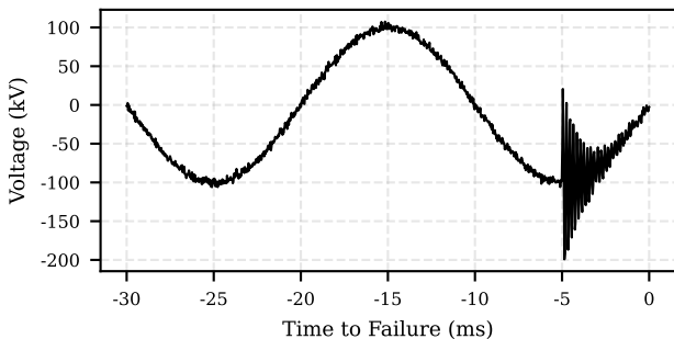
Micro Scale: Last 30 ms DFR (Algorithmic Autopsy)
