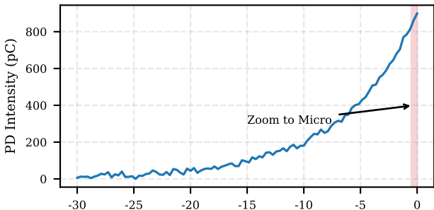
Meso Scale: Last 30 Days PD (Exponential Burst)
