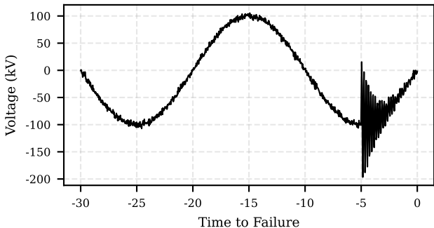
Micro Scale: Last 30 ms DFR (Algorithmic Autopsy)
