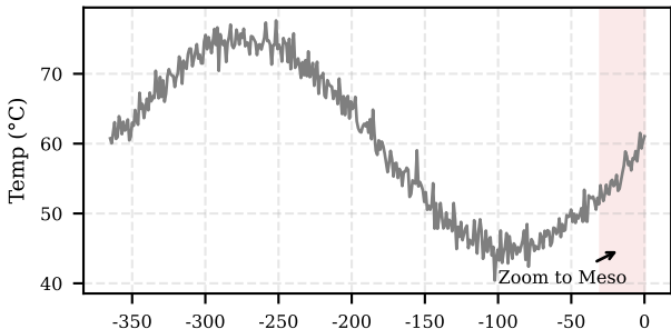
Macro Scale: 1 Year SCADA (Slow Drift)
