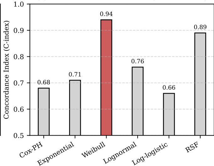
(b) GIS "6-Mirror" Evaluation (Weibull Wins)
