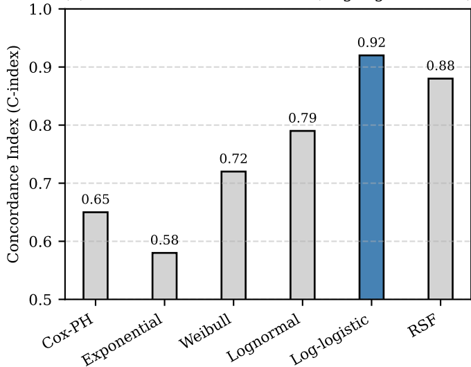
(a) AIS "6-Mirror" Evaluation (Log-logistic Wins)
