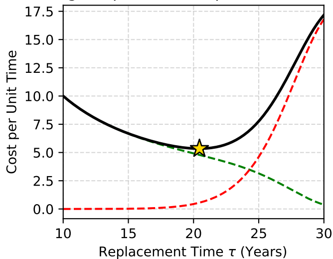
(b) Age Replacement Optimal Cost Curve
