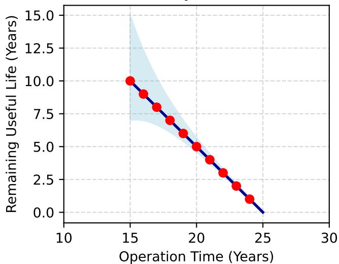
(a) 10-Decile Bayesian Error Funnel
