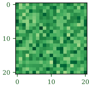
Head 8 Attention
