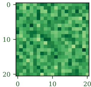
Head 4 Attention
