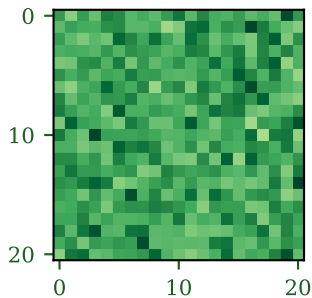
Head 2 Attention
