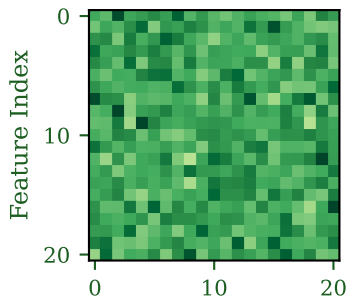
Head 5 Attention
