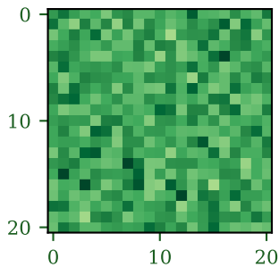
Head 6 Attention
