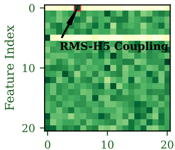
Head 1 Attention
