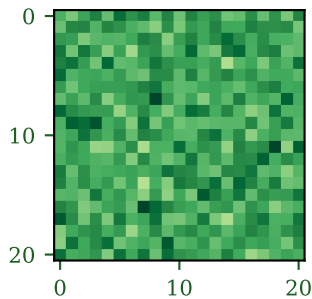
Head 7 Attention
