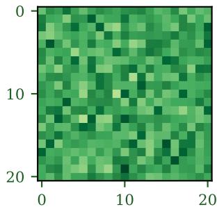
Head 3 Attention
