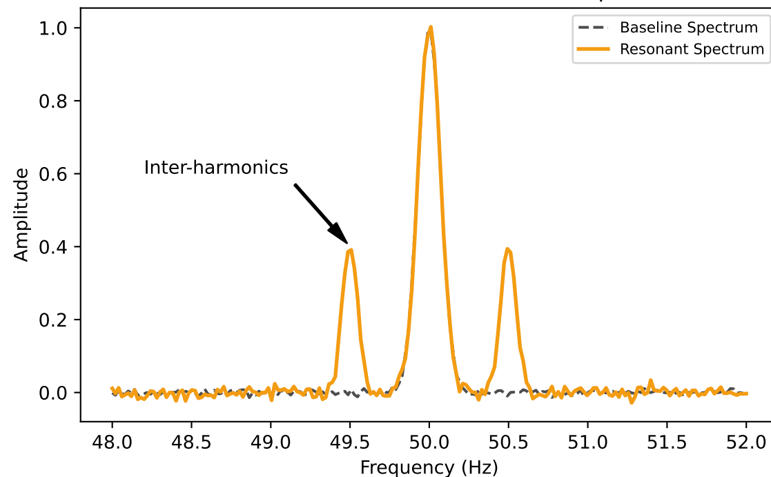
Scenario 3: Tower Resonance (Node A Spectrum)
