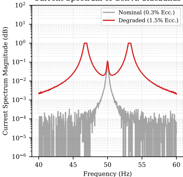
Current Spectrum of Gen A: Sidebands
