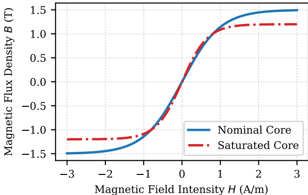
Transformer C Core B-H Curve
