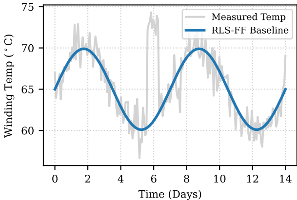
Online Baseline Calibration tracking (RLS-FF)
