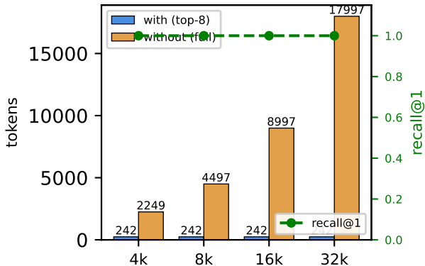
RULER NIAH retrieval efficiency (synthetic, lexical)
