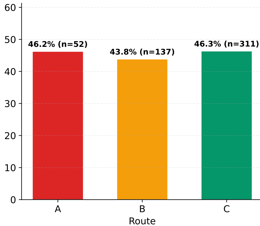
HotpotQA
