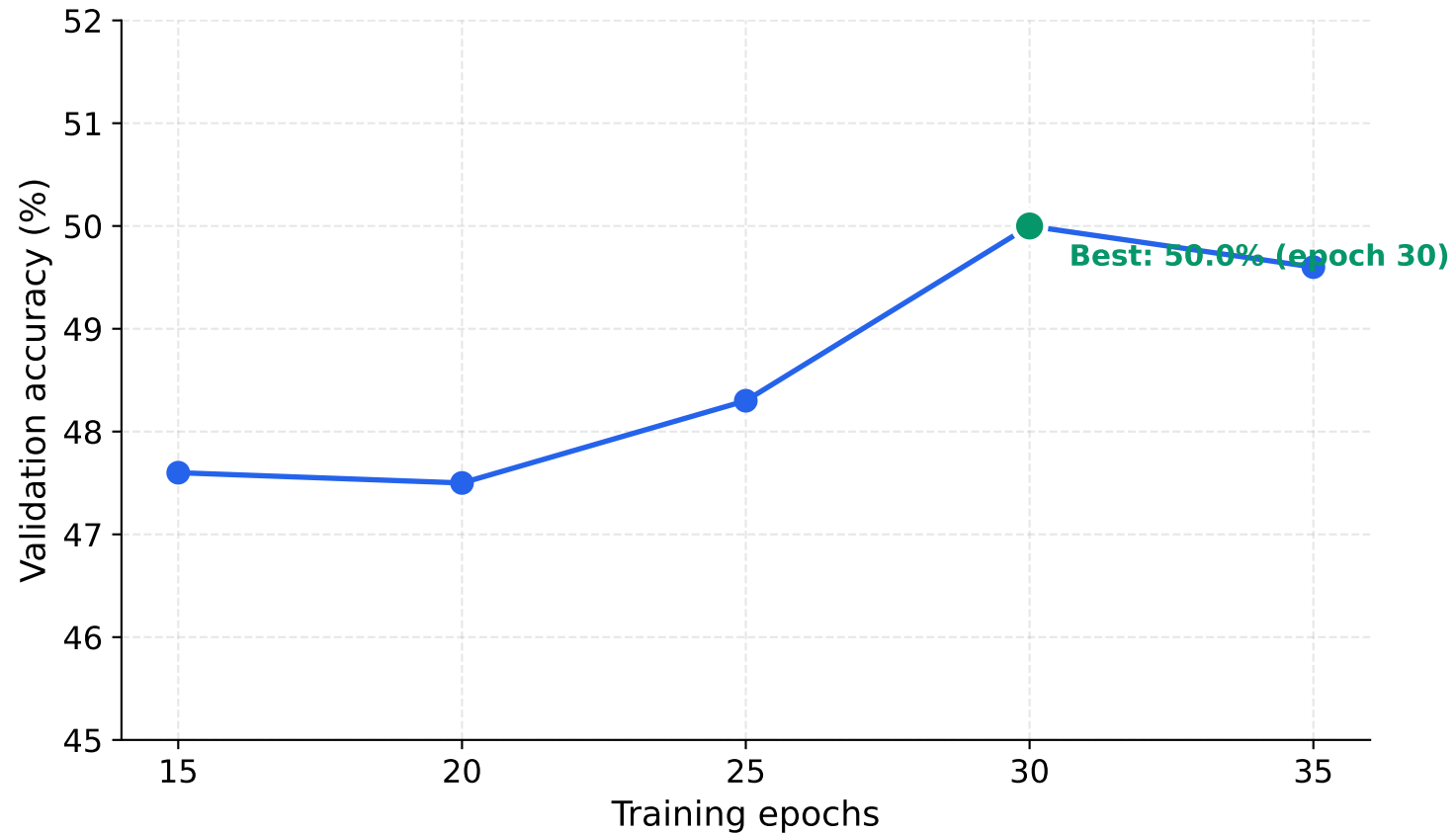
Classifier training: validation accuracy vs epochs
