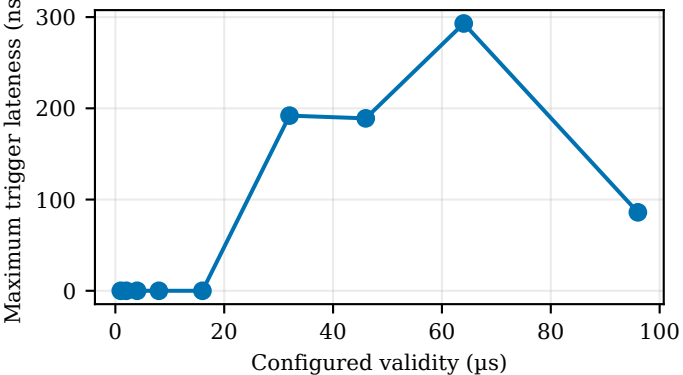
(a) Device-latency sweep
