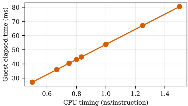
(b) CPU-rate sweep
