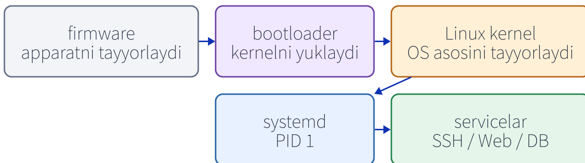
1-3-rasm. Kernel user space dagi birinchi processni ishga tushiradi, systemd esa kerakli service processlarini belgilangan tartibda boshlaydi.
