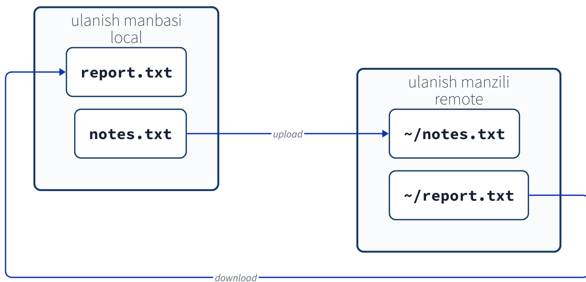
12-2-rasm. Upload va download command bajarilayotgan tomon nuqtayi nazaridan farqlanadi.
