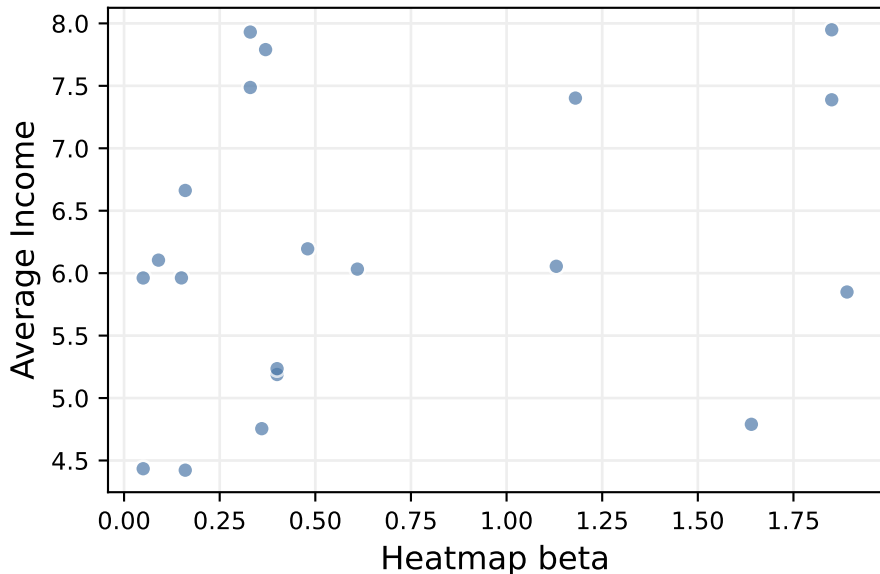
Global SA: Heatmap beta vs. Average Income
