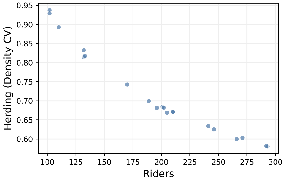
Global SA: Riders vs. Herding (Density CV)
