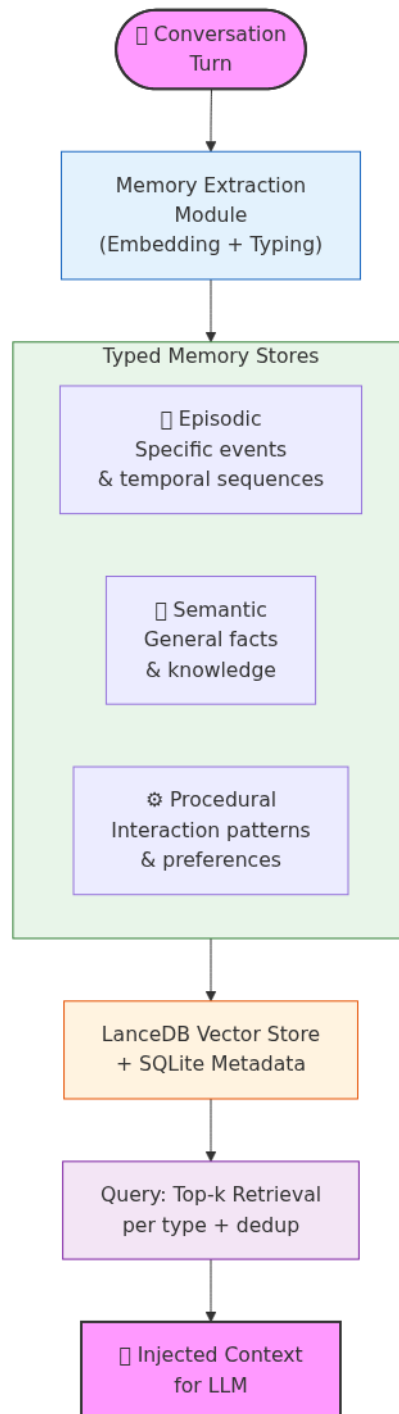
Figure 3: Typed memory architecture: Conversation \rightarrow Extraction \rightarrow Typed Stores (Episodic/Semantic/Procedural) \rightarrow Retrieval \rightarrow LLM Context.[4, 5] 8
