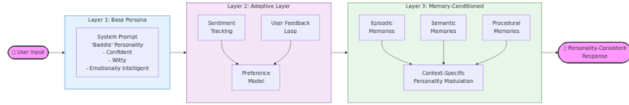
Figure 2: Three-layer personality modelling pipeline: Base Persona → Adaptive Layer → Memory-Conditioned Layer.[4, 5]abel{fig:personality}
