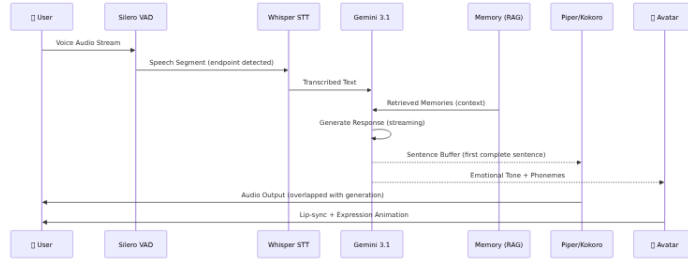
Figure 4: Voice interaction sequence: User → VAD → Whisper STT → LLM → TTS/Avatar with streaming overlap.[4, 5]abel{fig:voice}
