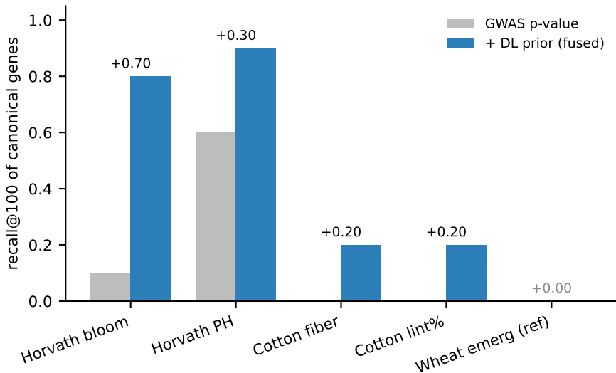
Fig 2 — DL-prior lift is panel-size / baseline-power dependent
