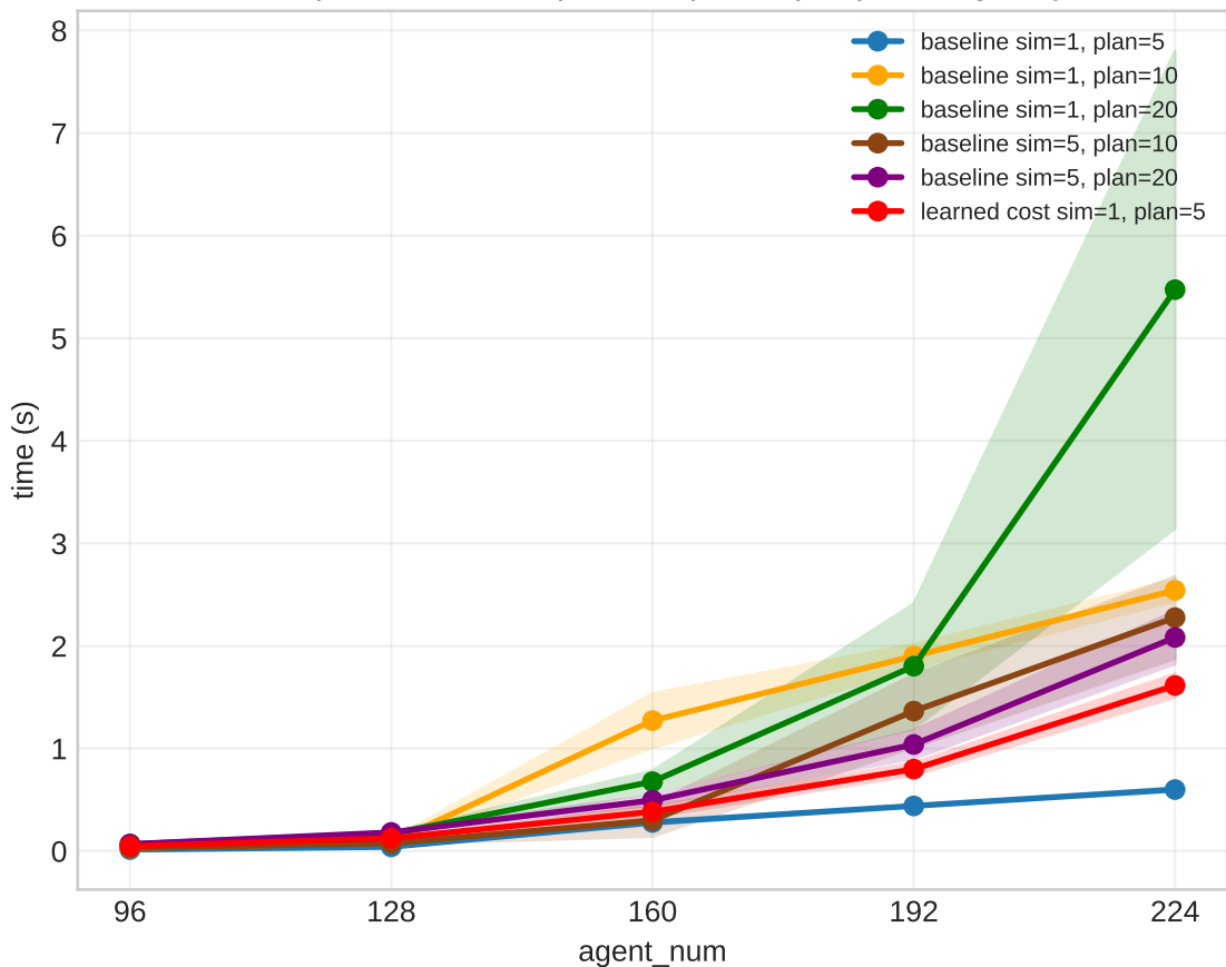
Compute Time Comparison (mean per planning call)
