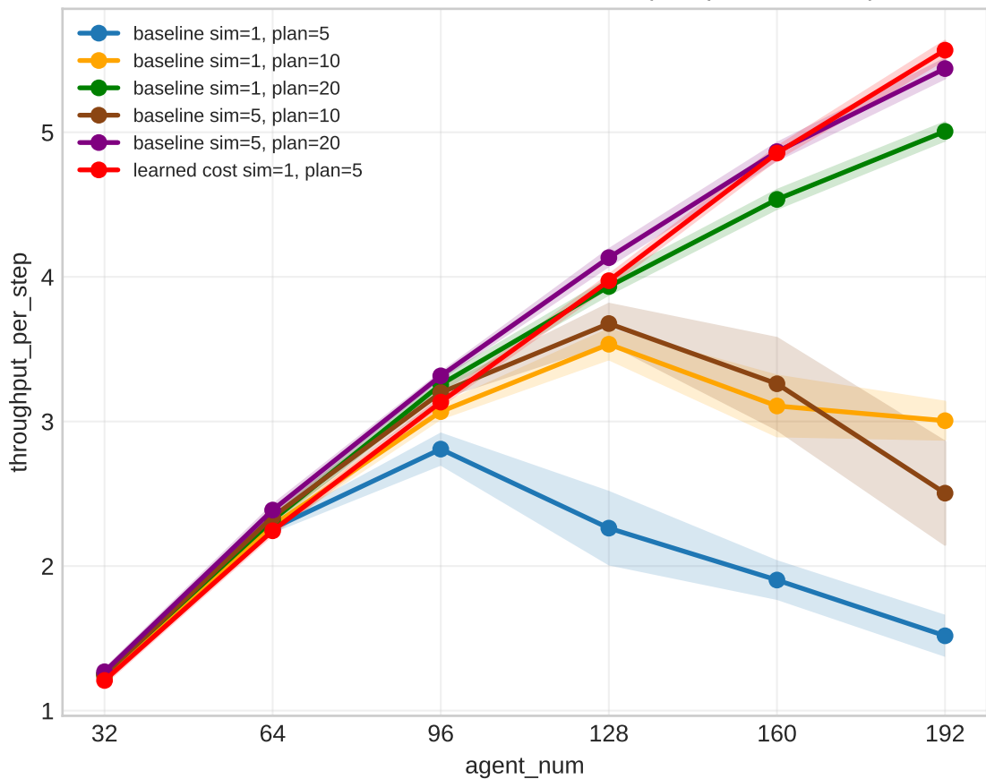
RHCR Combined: learned + baseline(sim/plan variants)
