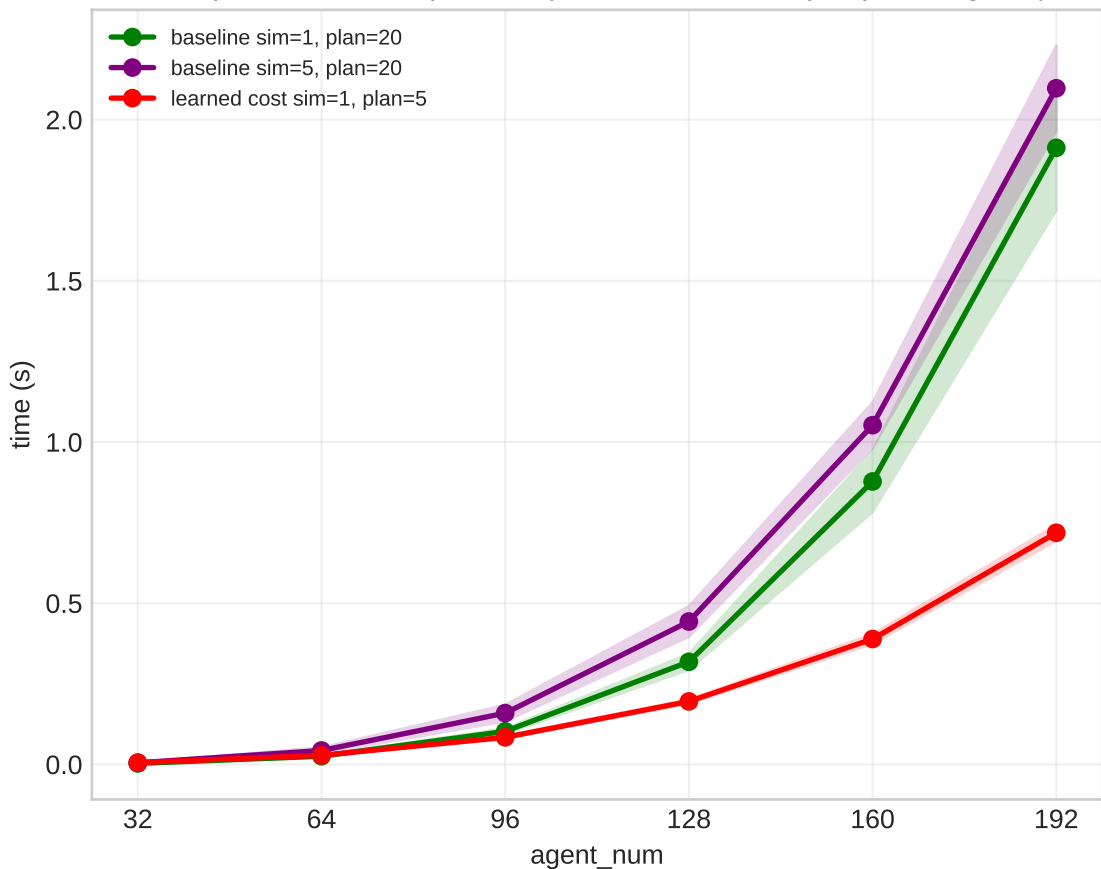
Compute Time Comparison (mean solver time per planning call)
