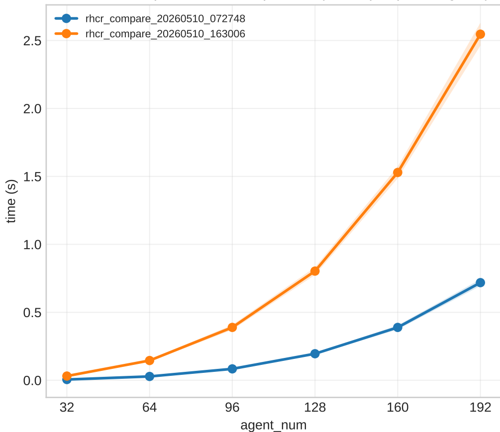
Learned Compute-Time Comparison (mean per planning call)
