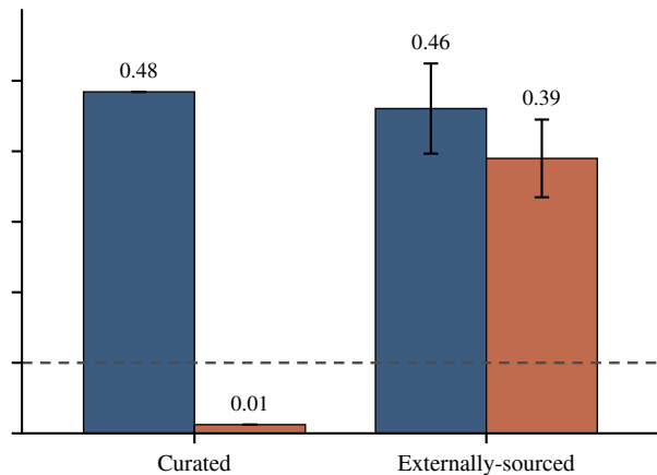
DistilBERT
