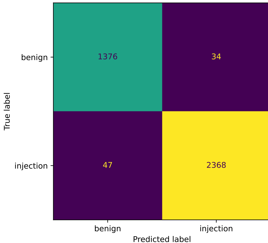
Confusion Matrix (DistilBERT, Test Set)
