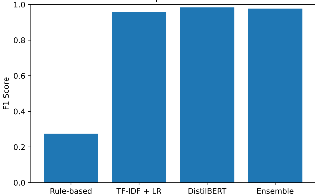
Model Comparison on Test Set
