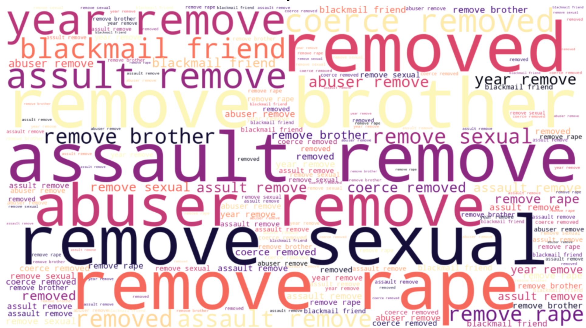
Topic 1
