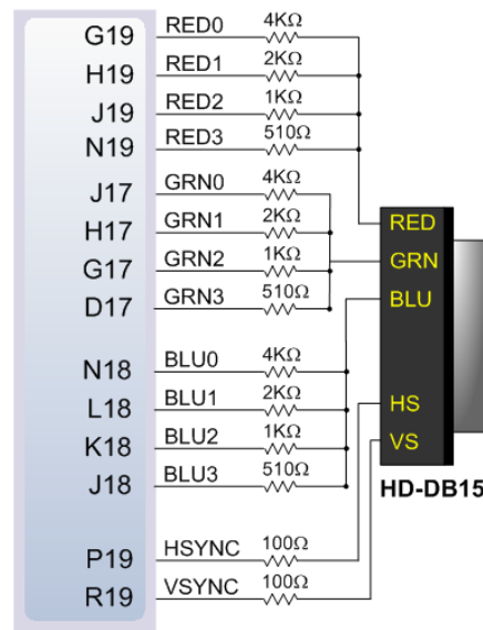
Artix-7
