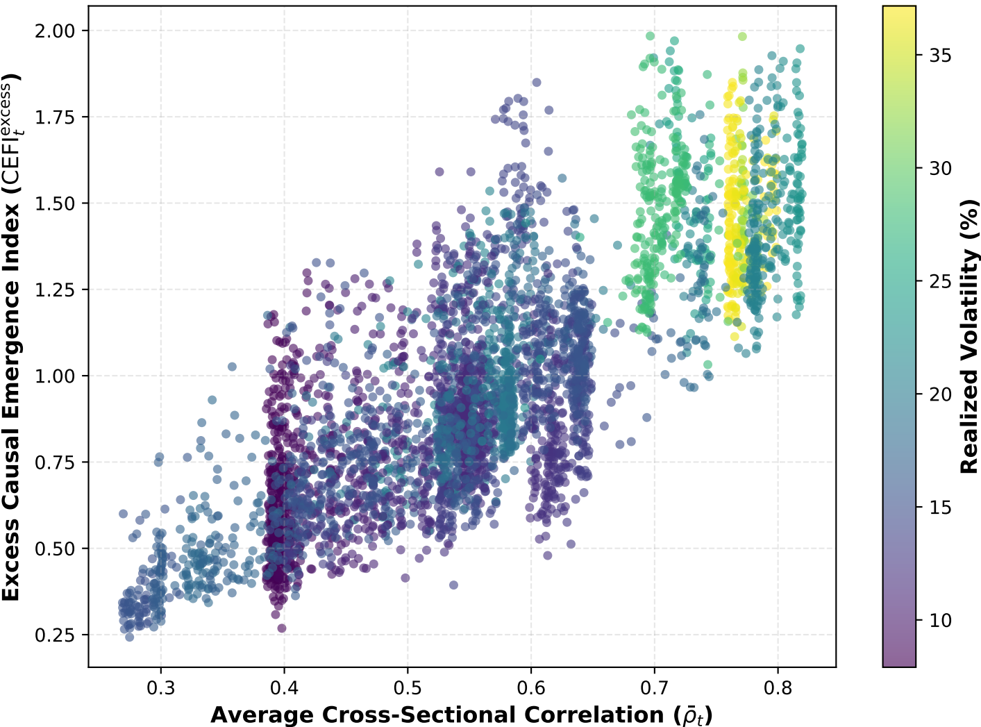
Non-Collinearity Analysis: \text{CEFI}_t^{\text{excess}} vs. Average Pairwise Correlation
