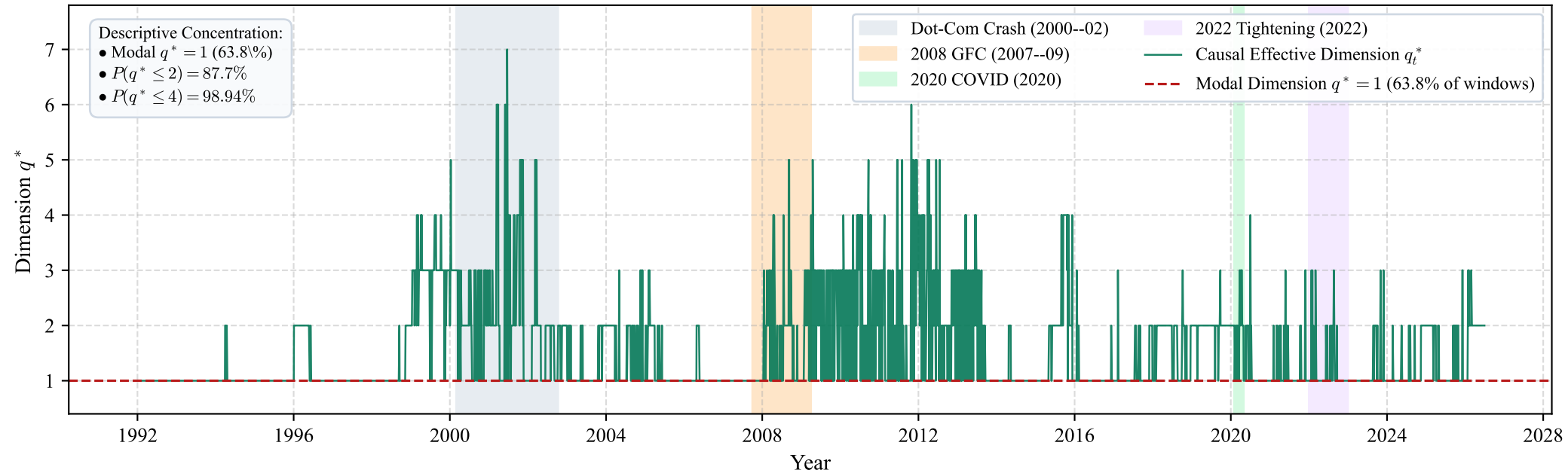
Evolution of Causal Effective Dimension ( q_t^* ) Across Market Regimes
