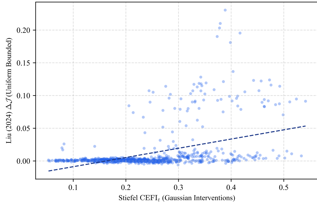
Stiefel (12/100) vs. Liu et al. (2024) (Pearson \rho = 0.445 , Spearman \rho_S = 0.356 )
