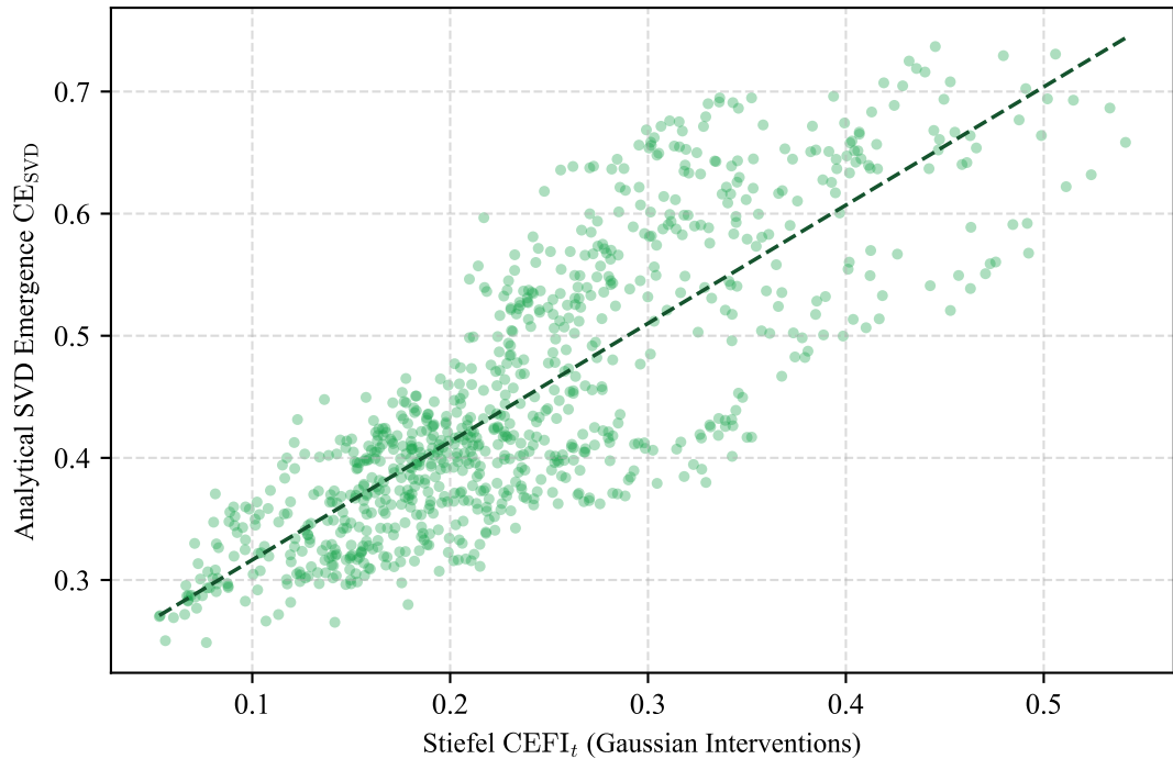
Stiefel (12/100) vs. Liu et al. (2025) SVD Emergence (Pearson \rho = 0.819 , Spearman \rho_S = 0.821 )
