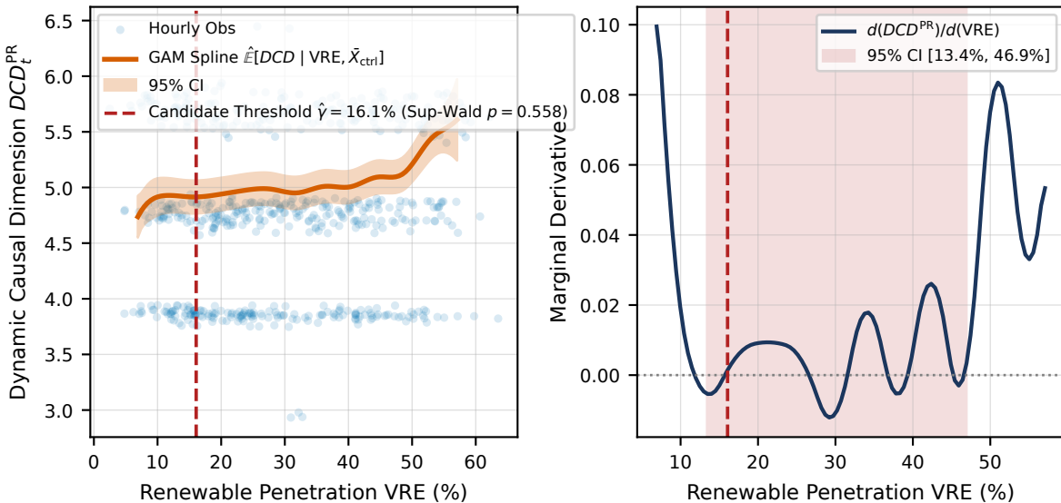
a | Nonlinear Causal Response to VRE (ERCOT) | Marginal Sensitivity & Hansen Sup-Wald Search
