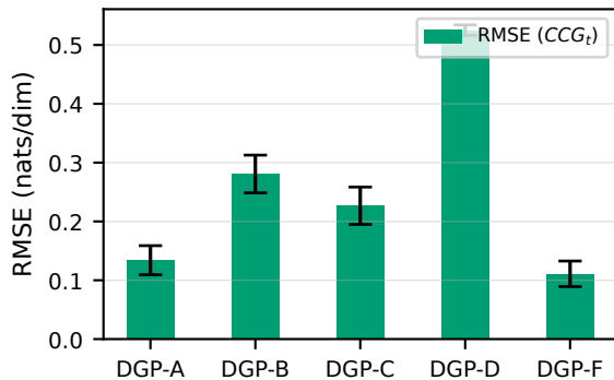
d | Tracking Error Across Benchmark DGPs
