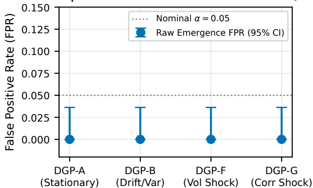
c | False Positive Rate under Nulls (R=100)
