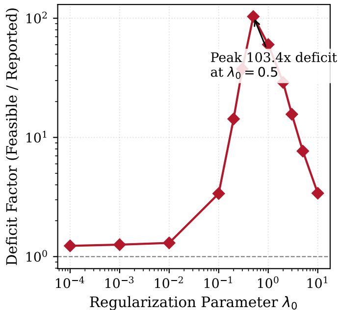
(b) Optimization Deficit Ratio
