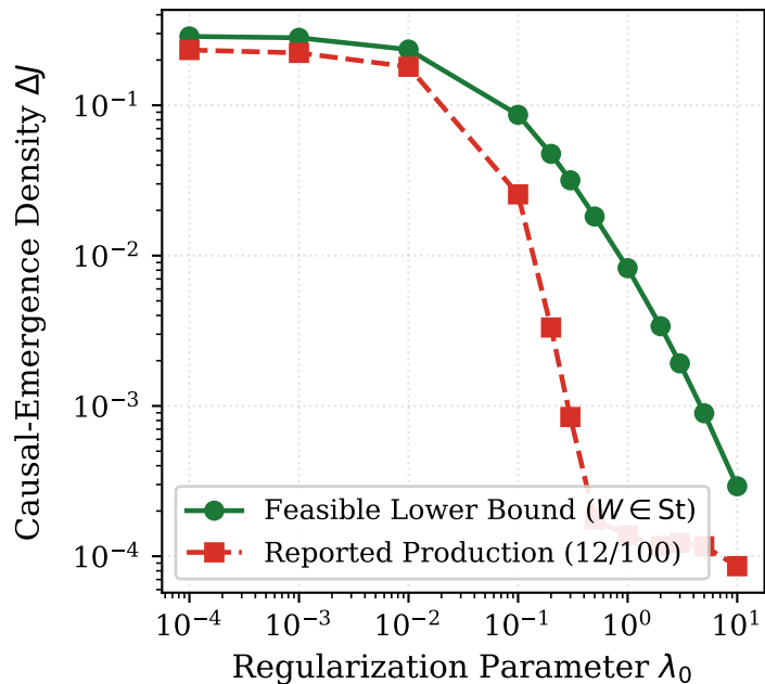
(a) Feasible-Witness Suboptimality Certificate
