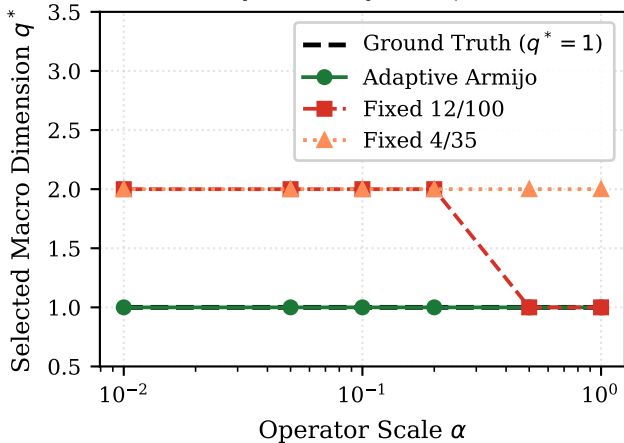
(a) Synthetic System ( p = 30 )
