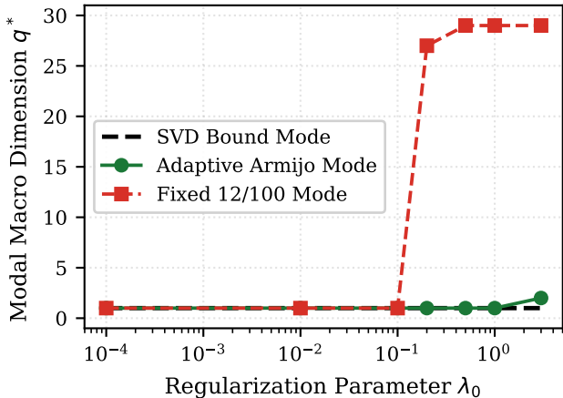
(b) Empirical Trajectory ( p = 30 )
