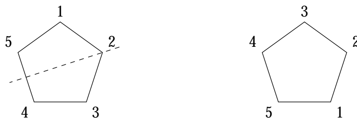
Figure 6.1.2 The reflection \begin{smallmatrix} 1 & 2 & 3 & 4 & 5 \\ 3 & 2 & 1 & 5 & 4 \end{smallmatrix} .
