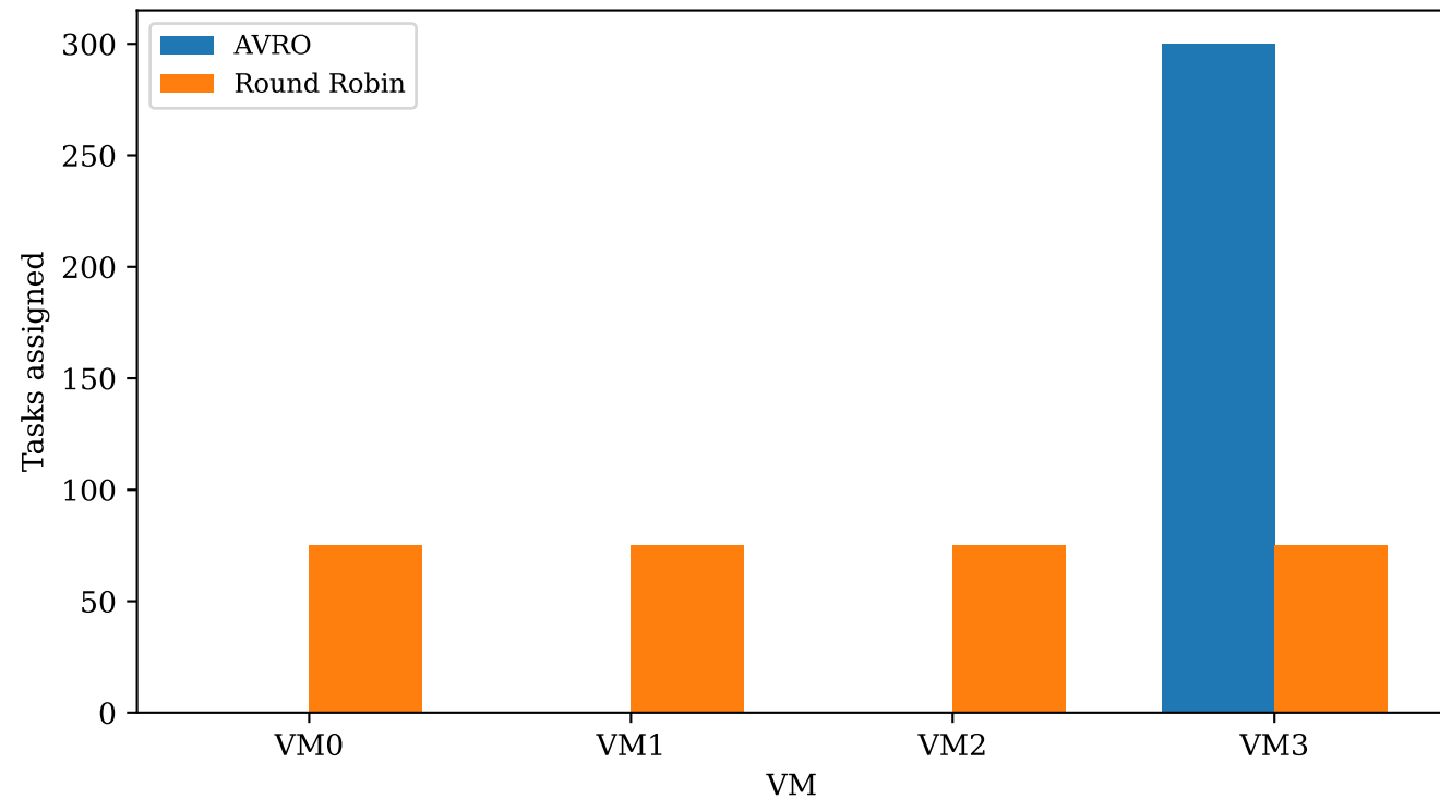
VM Selection Distribution
