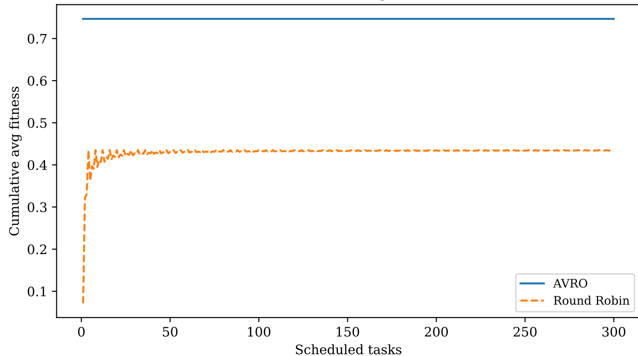
Cumulative Average Fitness
