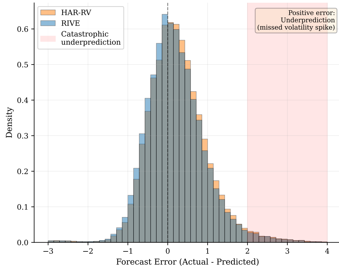
Distribution of Forecast Errors
