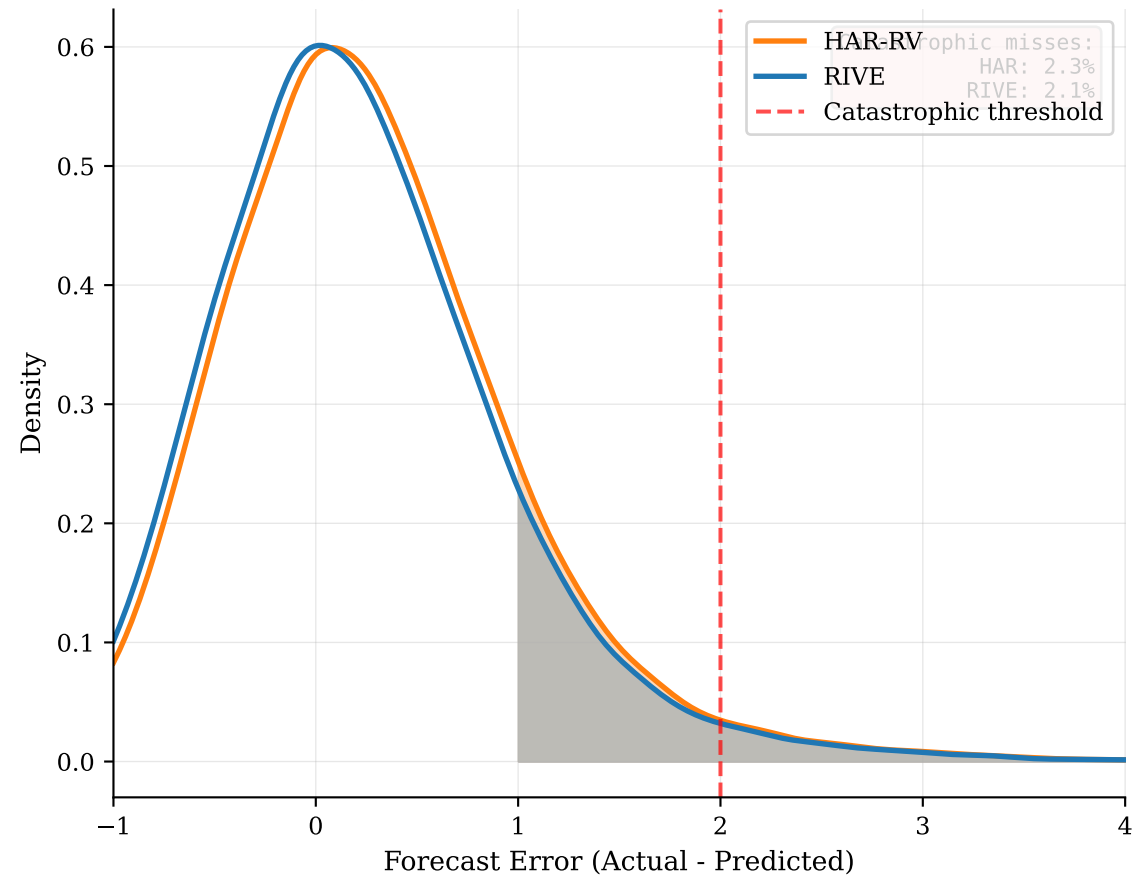
Right Tail Detail (Underprediction Risk)
