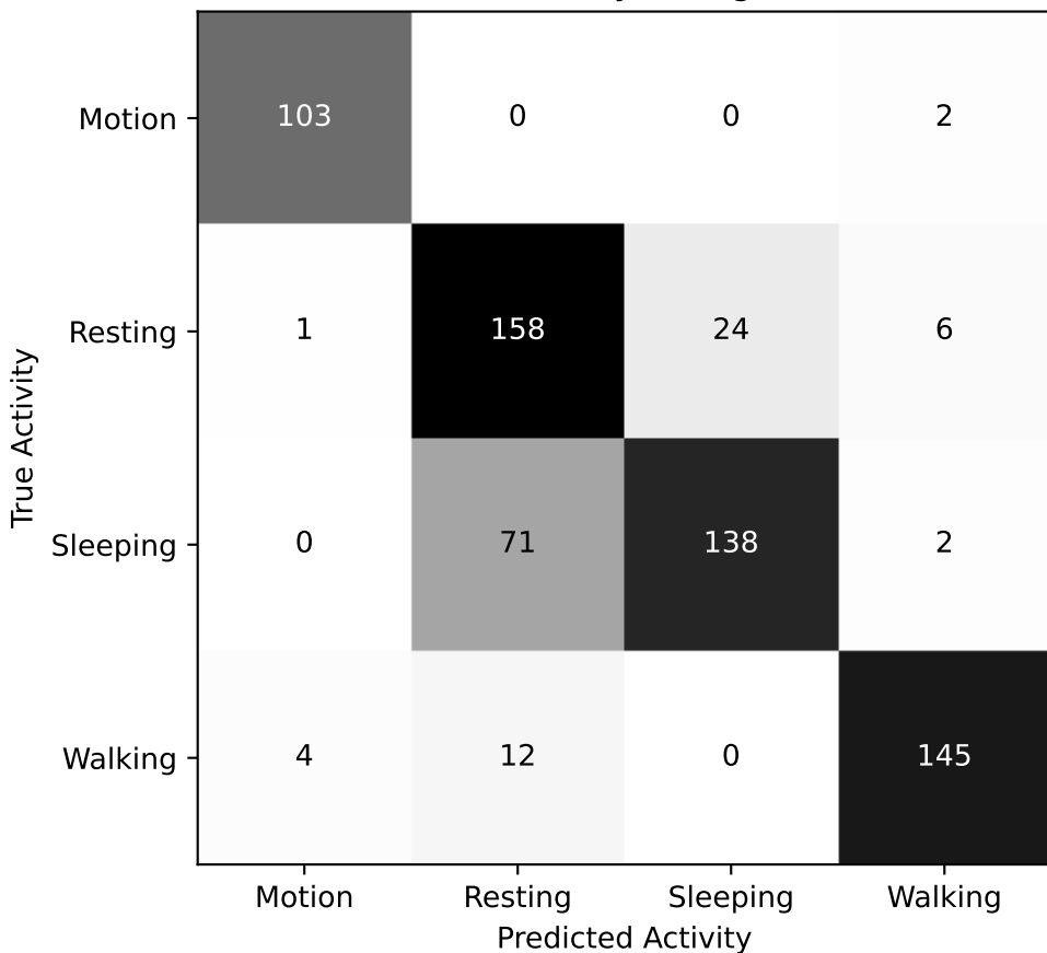
LOSO Activity Recognition
