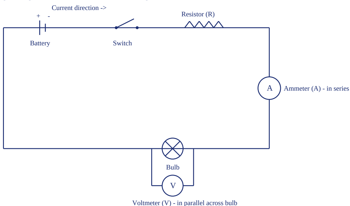
Fig. 1 - Circuit diagram
