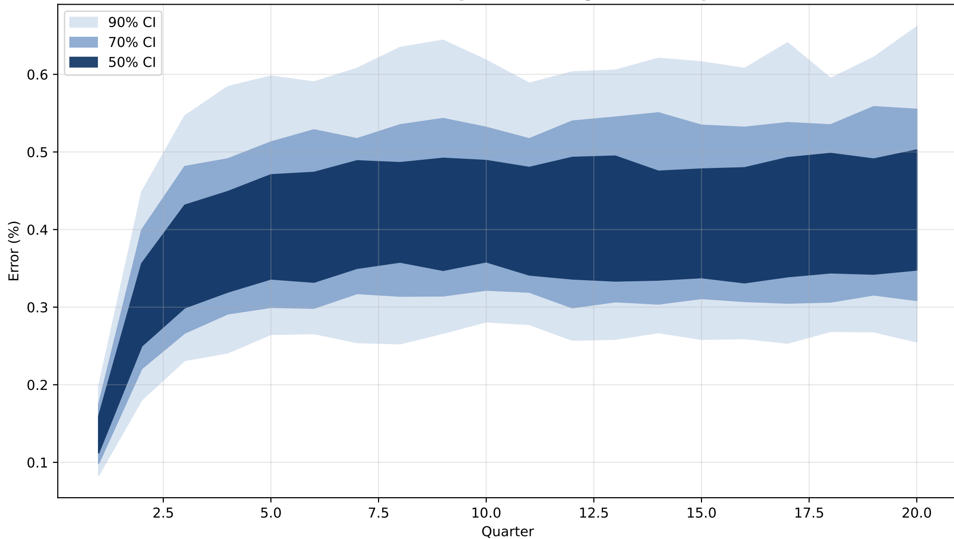
Monte Carlo: Alpha Tracking Error (Gap)
