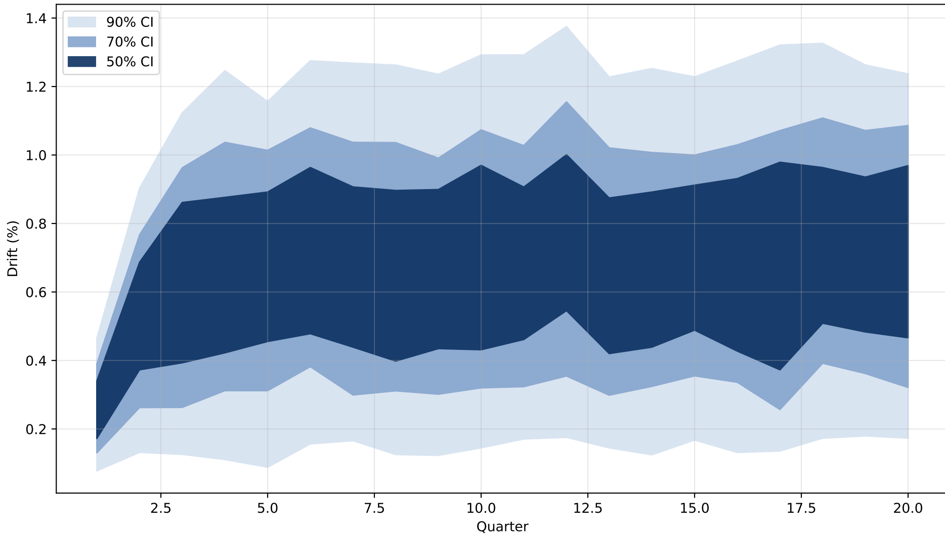
Monte Carlo: Price Drift (RMS)
