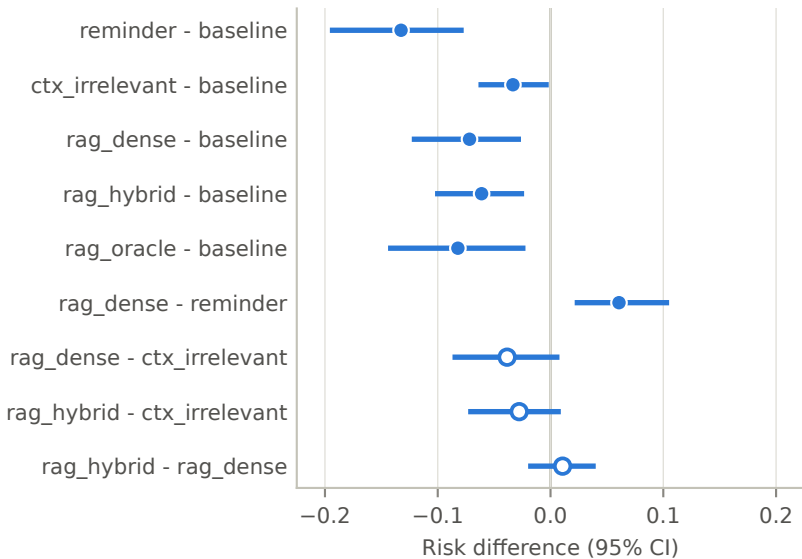
Change in vulnerable answers
